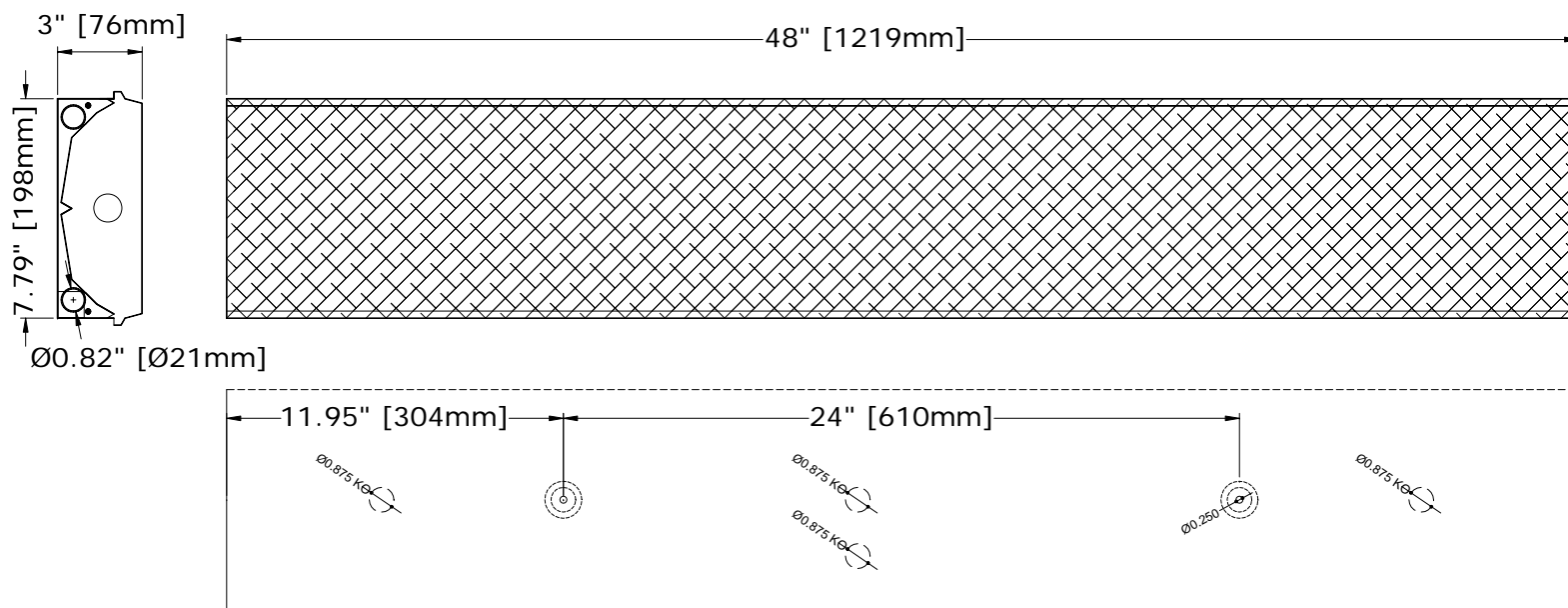
BACK SIDE VIEW
